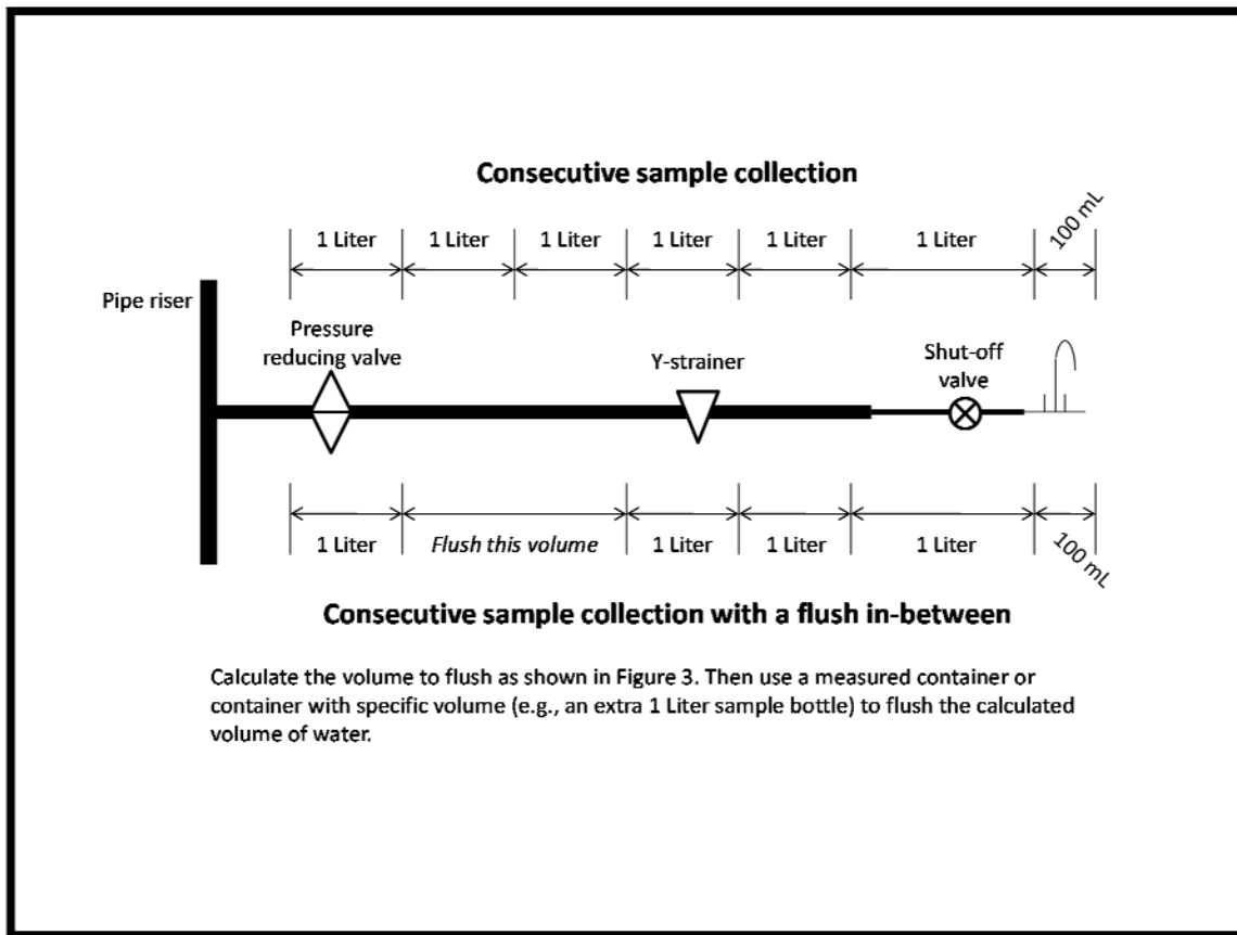
Figure 6. Examples of Consecutive Sampling and Flushing between Sampling
