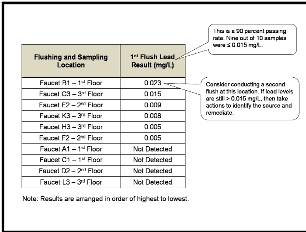
Figure 3. Example of 90 Percent Passing Rate after First Flush.
